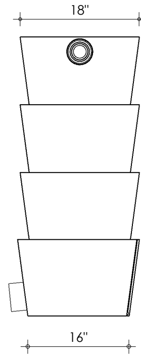
Right-side view
